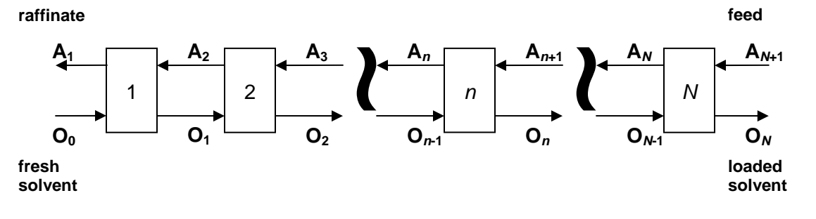
Figure 1. Countercurrent – multistage extraction process flow diagram
