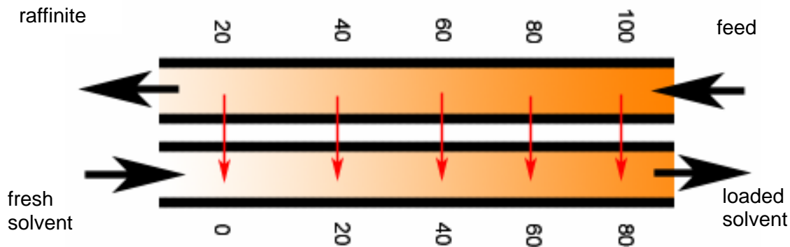
Figure 2. Countercurrent process concentration profiles
