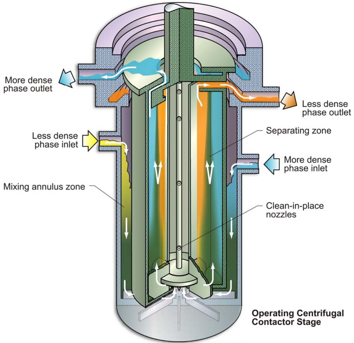
Figure 5. Cutaway view of an operating centrifugal contactor
